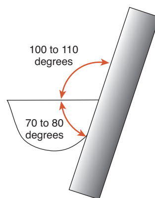
eFig. 50.60 When the sharpening stone forms a 100- to 110-degree angle with the face of the blade, the 70- to 80-degree angle between the face and the lateral surface is automatically preserved.
