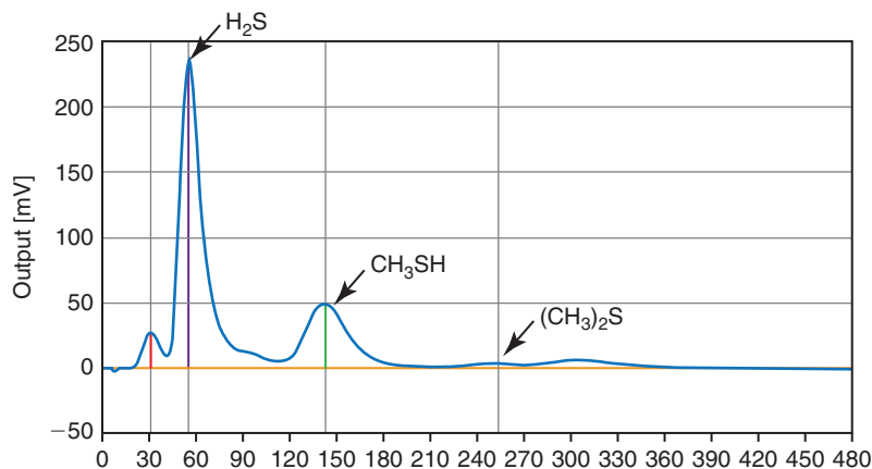
Fig. 49.8 Graphic from the OralChroma. The first peak indicates the level of hydrogen sulfide (HS), the second the level of methylmercaptan (CHSH), and the third the level of dimethyl sulfide ((CH 3 ) 2 S). 2332
