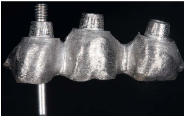
Fig. 77.10 During the fabrication of a screw-retained PFM, the technician must exercise extreme care in creation of the framework so as not to damage the interface area as shown here. The damaged interface will produce a poor-fitting prosthesis leading to increased leakage and screws that loosen more frequently.
