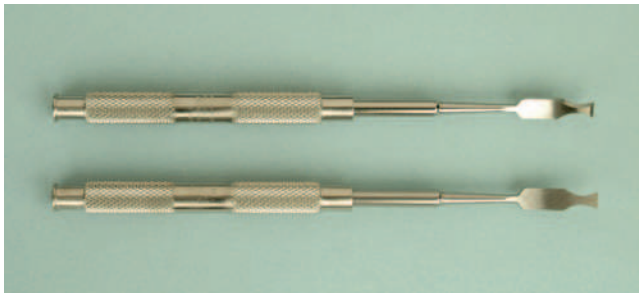
Fig. 59.11 Ochsenbein chisels are paired, with their cutting edges in opposite directions.
