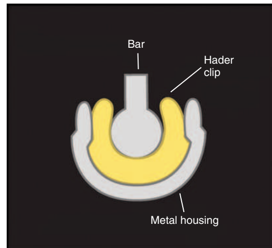
eFig. 77.17 Cross section of a Hader bar with clip. Note that the minimal height of the Hader bar is 2.5 mm and about 1.2 mm for the plastic clip and the metal housing. We should also allow room for acrylic for the retention of these components.
