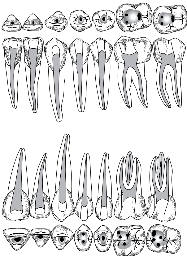
Fig. 8.1 Access cavity preparations.
