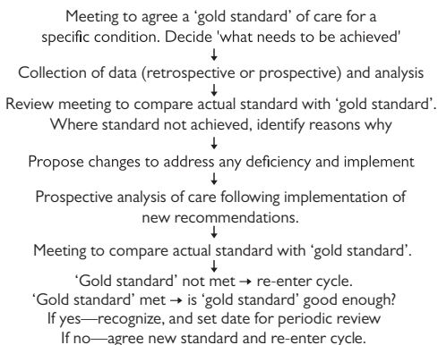
Fig. 19.1 Audit cycle.
