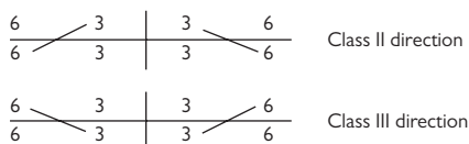
Fig. 4.13 Reinforcing anchorage.
