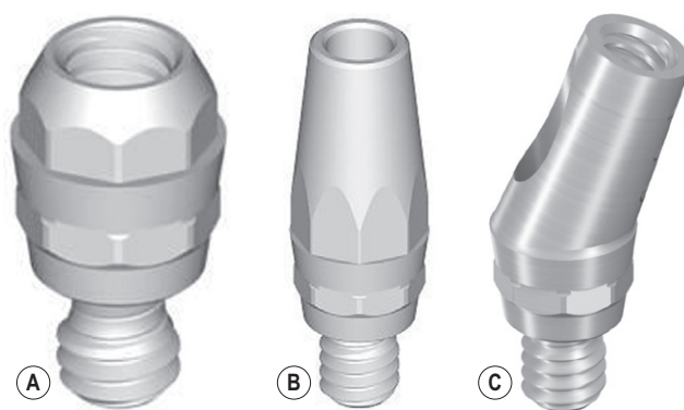
Fig 21.10 Prefabricated (A) screw-retained abutment, (B) straight-cemented abutment, and (C) angled abutment.
